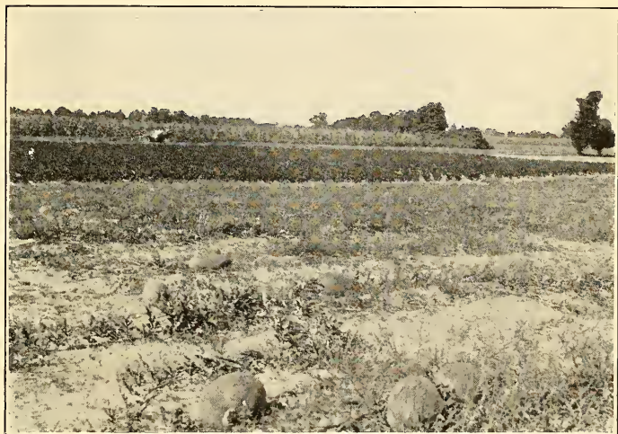
FIG. 29. — WATERMELONS, PEPPERS AND CORN FERTILIZED WITH BASIC FERTILIZER, CLARKSBORO, NEW JERSEY.
